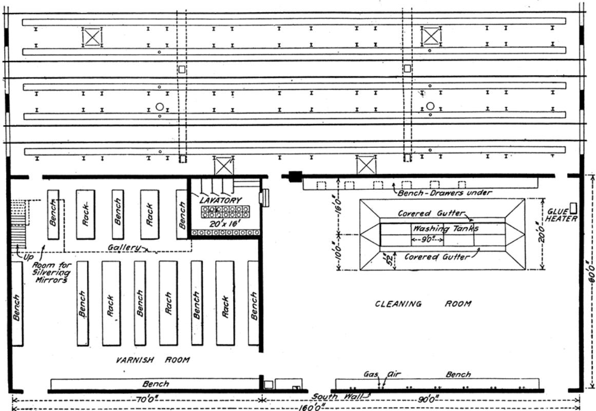
PARTIAL PLAN OF PASSENGER CAR PAINT SHOP AT COLLINWOOD, OHIO, L. S. & M. S. RY.
