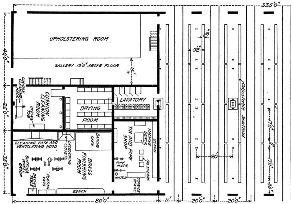
PARTIAL PLAN OF PASSENGER CAR REPAIR SHOP AT COLLINWOOD, OHIO, L. S. & M. S. RY.
