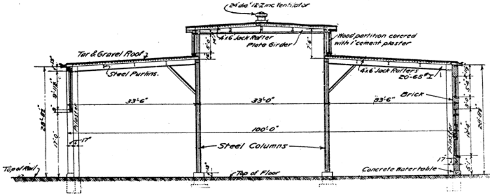
CROSS SECTION OF PAINT SHOP AT SEDALIA, MO., M. P. RY.
