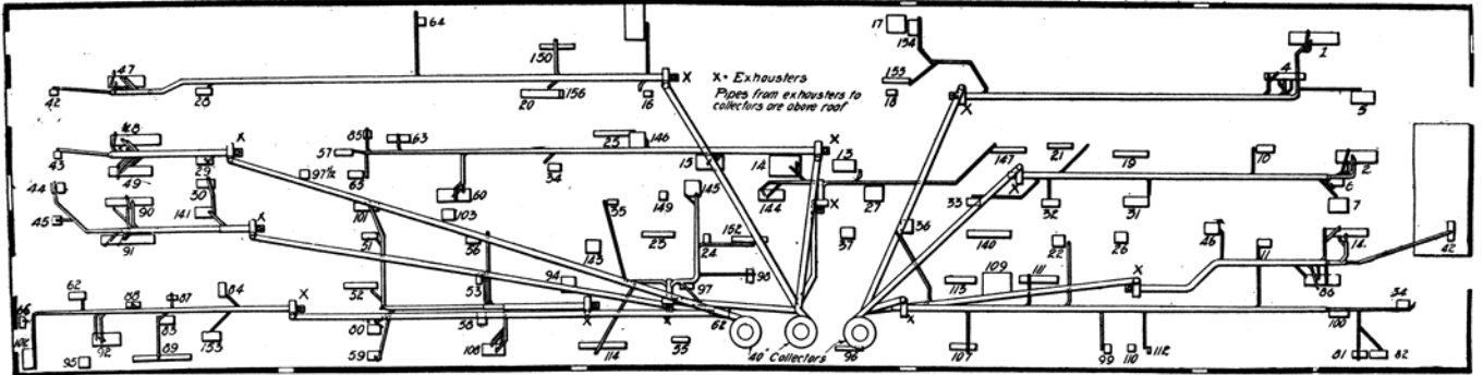
PLAN OF PLANING MILL, SHOWING ARRANGEMENT OF SHAVINGS EXHAUST DUCTS, AT ANGUS, C. P. RY.
