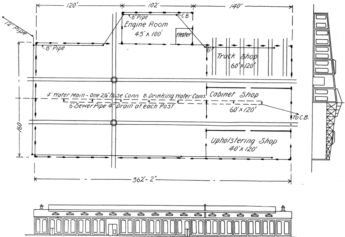
PLAN, ELEVATIONS AND PARTIAL CROSS SECTION OF PLANING MILL AT BURNSIDE, ILL., I. C. R. R.
