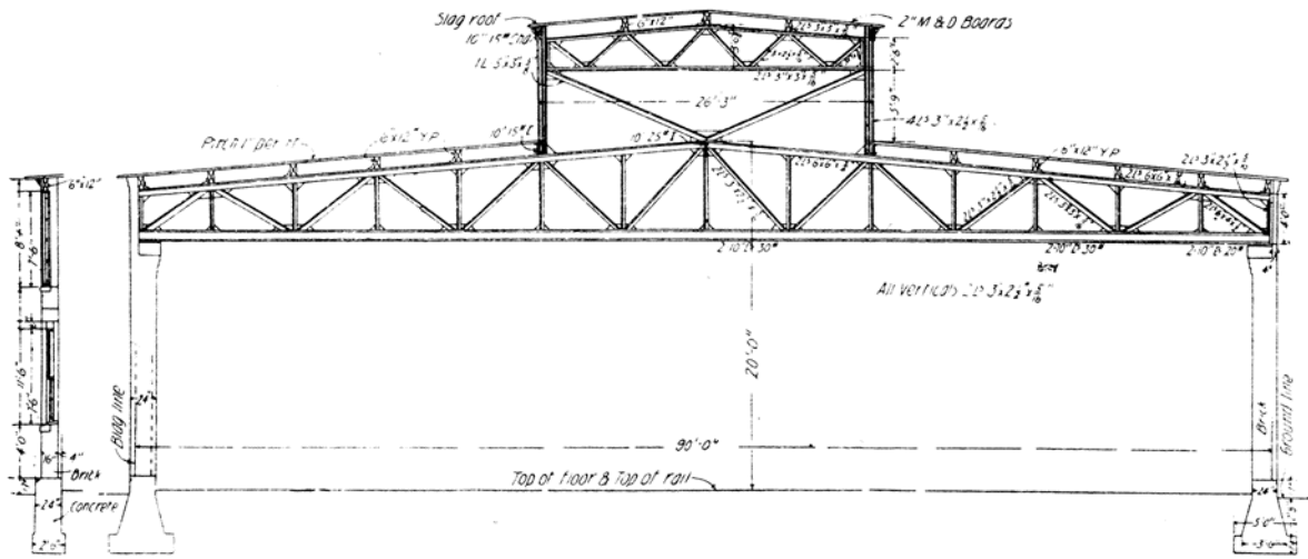
CROSS SECTION OF PLANING MILL AT SCRANTON, PA., D. L. & W. R. R
