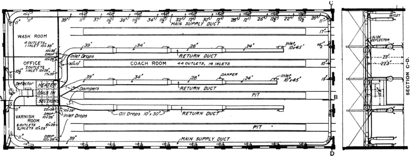
ARRANGEMENT OF HEATING SYSTEM IN PAINT SHOP AT McKEES ROCKS, PA., P. & L. E. R. R.
