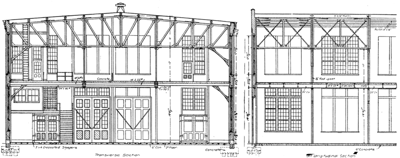
SECTION OF PLANING MILL AND COACH SHOP AT SOUTH LOUISVILLE, KY., L. & N. R. R.
