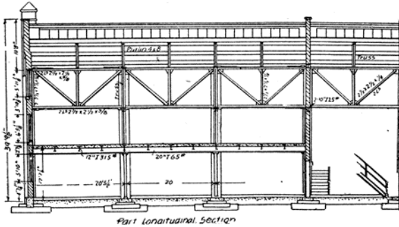
PARTIAL LONGITUDINAL SECTION OF PASSENGER COACH AND PAINT SHOP AT SOUTH LOUISVILLE, KY., L. & N. R. R.
