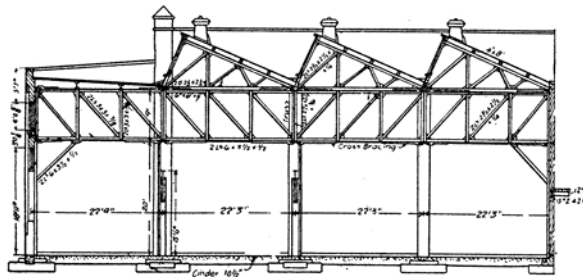
PARTIAL CROSS SECTION OF PASSENGER COACH AND PAINT SHOP AT SOUTH LOUISVILLE, KY., L. & N. R. R.
