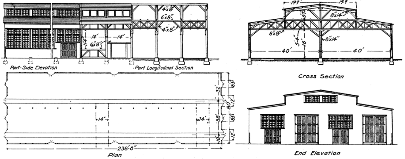
PLAN, ELEVATIONS AND SECTIONS OF PLANING MILL AT EAST DECATUR, ILL., WABASH R. R.
