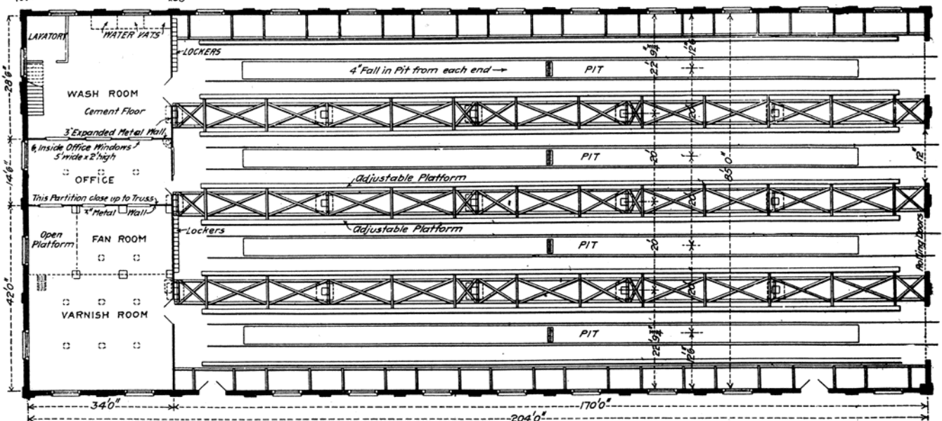
PLAN, PARTIAL SECTION AND ELEVATION OF PASSENGER CAR PAINT SHOP AT McKEES ROCKS, PA., P. & L. E. R. R.
